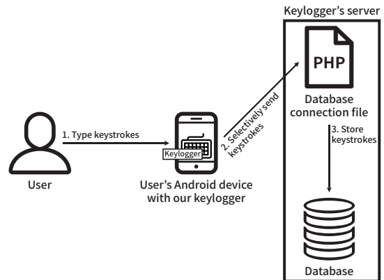
Fig. 1: Overview of our proof-of-concept keylogging system
