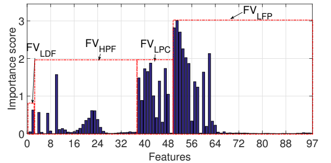
Figure 7: Importance scores for individual features on the ASVspooft dataset.
